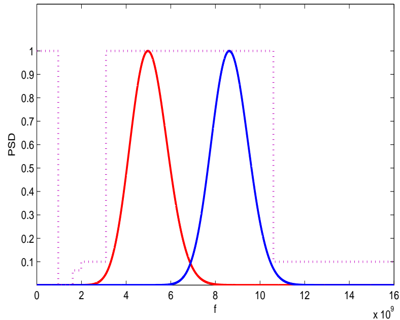
Figure 81: GFSK UWB Mask normal scale, 9 and 27 order \alpha = 0.34 ns
