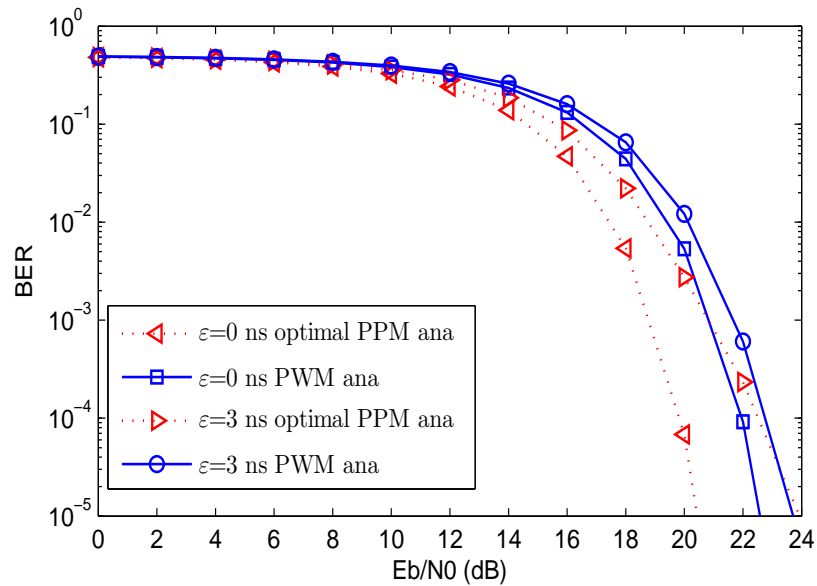
Figure 61: Comparison of BER performance of PWM and optimal threshold PPM systems in multipath channels (CM4 model, D=80 ns, \epsilon=0 and 3 ns)
