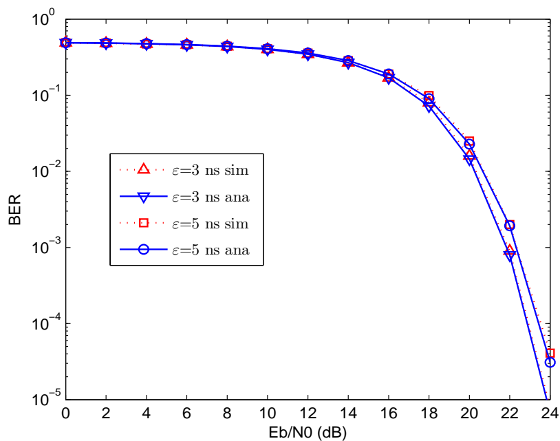
Figure 77: BER performance of PWM in multipath channels (CM4 model, \delta = D = 80 ns, \epsilon = 3 and 5 ns)
