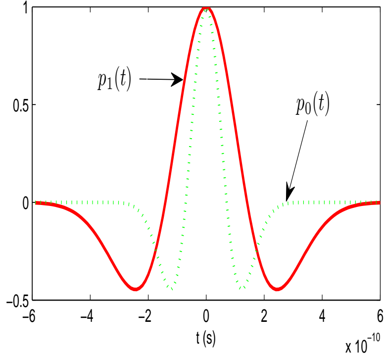
Figure 8: The waveform of the 2nd-order derivative of the Gaussian pulse with different shaping factors: \alpha_1 = 2\alpha_0
