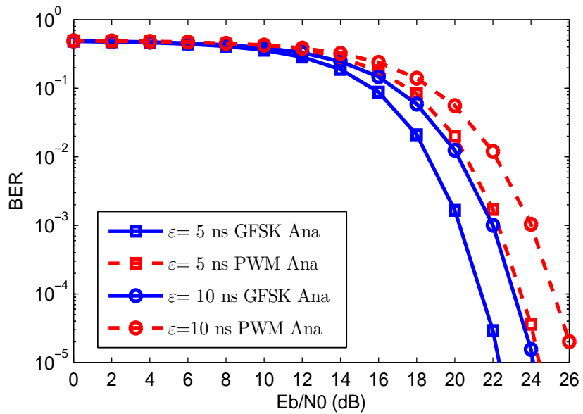
Figure 44: Comparisons of Analytical BER performance of PWM and GFSK in the presence of synchronization errors ( \epsilon = 5 ns and 10 ns)
