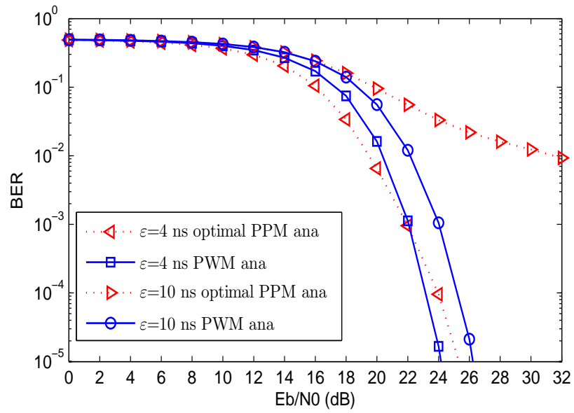
Figure 62: Comparison of BER performance of PWM and optimal threshold PPM systems in multipath channels(CM4 model, D=80 ns, \varepsilon =4 and 10 ns)
