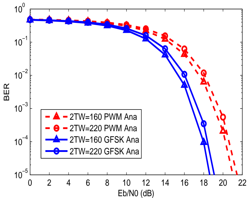
Figure 36: Comparisons of Analytical BER performance of PWM and GFSK in AWGN channels(2TW=160 and 220)
