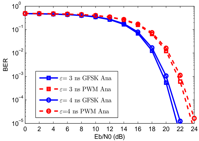
Figure 43: Comparisons of Analytical BER performance of PWM and GFSK in the presence of synchronization errors ( \epsilon = 3 ns and 4 ns)
