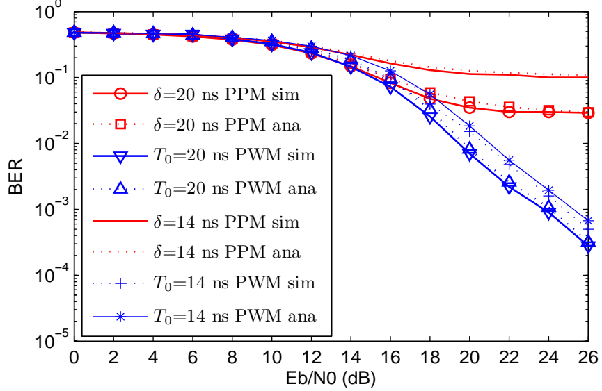
Figure 19: Comparison of BER performance of PWM and PPM in Multipath channels (CM4 model, \delta = 20 ns and 14 ns)
