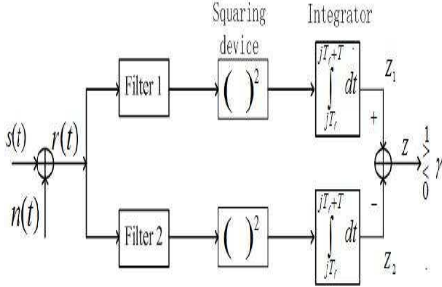
Figure 10: PWM Receiver
