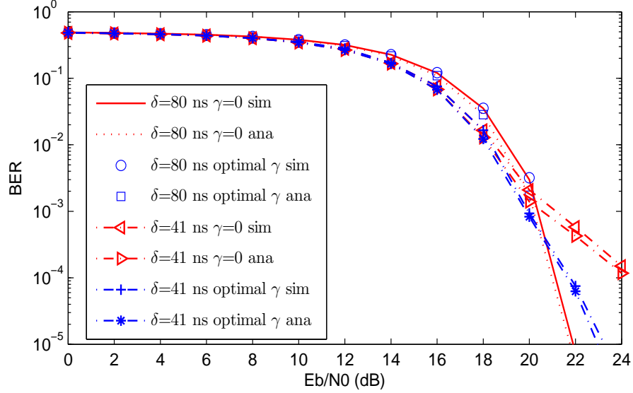
Figure 46: Comparison of BER performance of the 0 and optimal threshold PPM systems in multipath channels (CM4 model, D=80 ns, \delta =80 and 41 ns)
