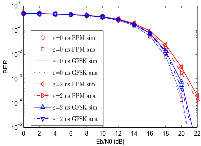
Figure 32: Comparisons of BER performance of GFSK and PPM in the presence of synchronization errors (CM4 model, \delta = D = 80 ns, \epsilon = 0 and 2 ns).
