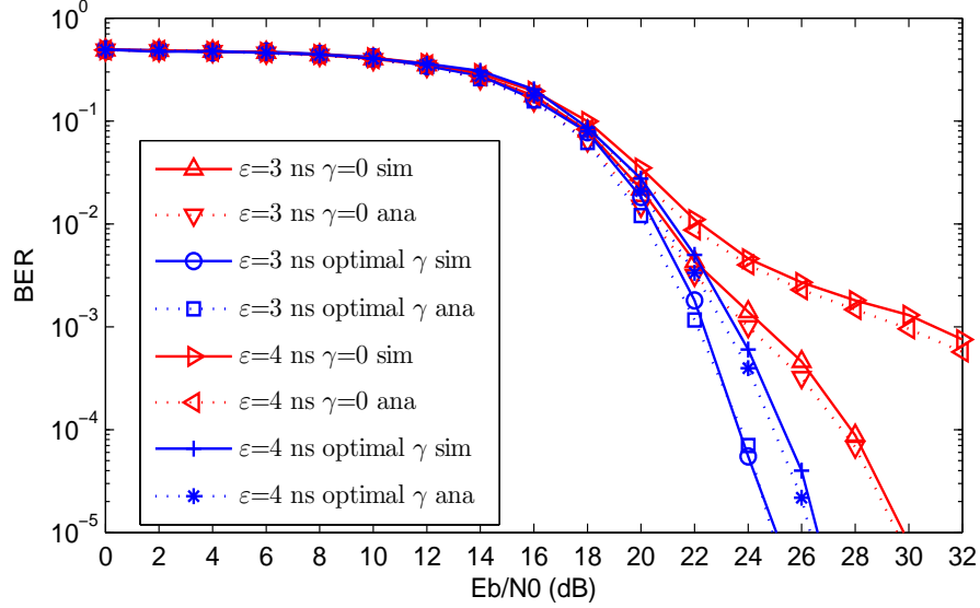
Figure 50: Comparison of BER performance of 0 and optimal threshold PPM systems in the presence of synchronization errors(CM4 model, D=80 ns, \varepsilon =3 and 4 ns)
