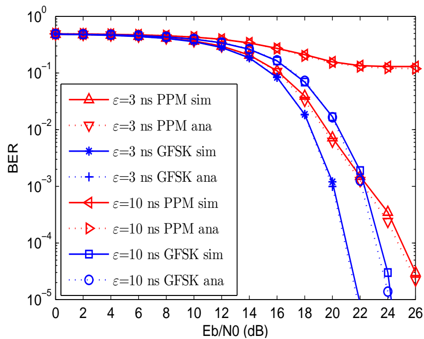
Figure 90: Comparison of BER performance of GFSK and PPM in multipath channels (CM4 model, D = 80 ns, \epsilon = 3 and 10 ns)
