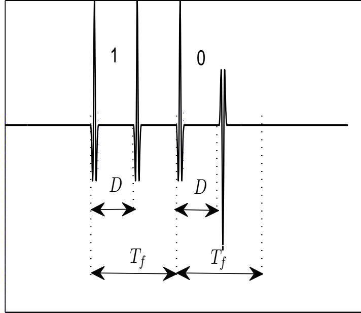
Figure 7: Frame structures of a transmitted reference system(from [9])
