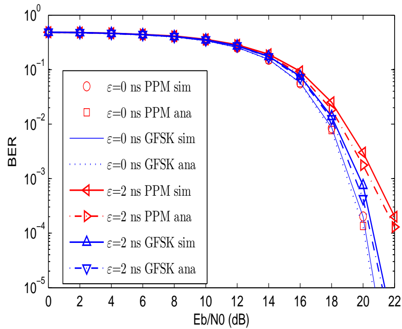
Figure 89: Comparison of BER performance of GFSK and PPM in multipath channels (CM4 model, D = 80 ns, \epsilon = 0 and 2 ns)
