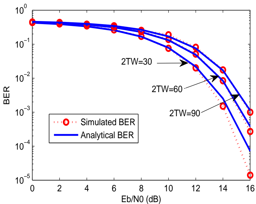
Figure 86: BER performance of GFSK for different 2TW values in AWGN channels
