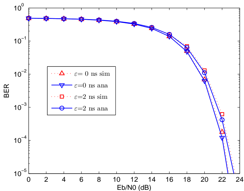
Figure 76: BER performance of PWM in multipath channels (CM4 model, \delta = D = 80 ns, \epsilon = 0 and 2 ns)
