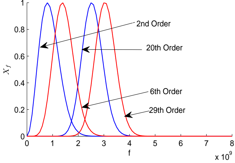
Figure 25: Spectra of two pulse pairs
