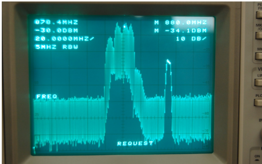
Fig. 3.2: The center frequency of the RF signal emitted by the cell phone used shows a reading of 878 MHz.
